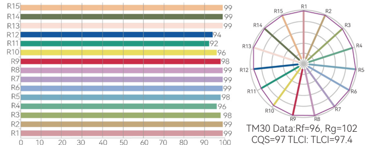
2835 DAYLIGHT COLOR RENDERING INDEX CCT 6498K Ra=98.4
